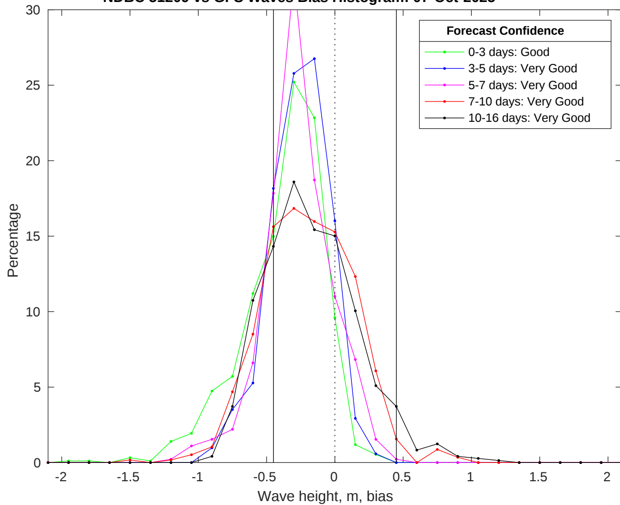
NDBC 51209 vs GFS Waves Bias Histogram: 07-Oct-2025
