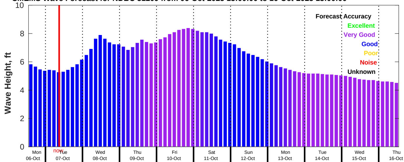
CMEMS Wave Forecast for NDBC 51209 from 06-Oct-2025 13:00:00 to 16-Oct-2025 13:00:00
