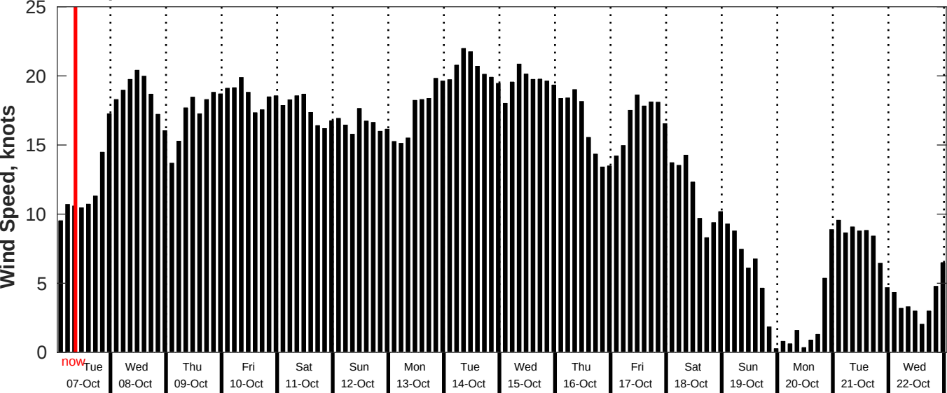
GFS Wind Speed Forecast for NDBC 51209 from 07-Oct-2025 01:00:00 to 23-Oct-2025 01:00:00
