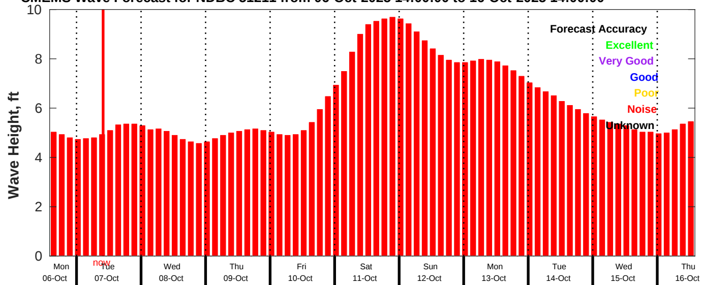
CMEMS Wave Forecast for NDBC 51211 from 06-Oct-2025 14:00:00 to 16-Oct-2025 14:00:00
