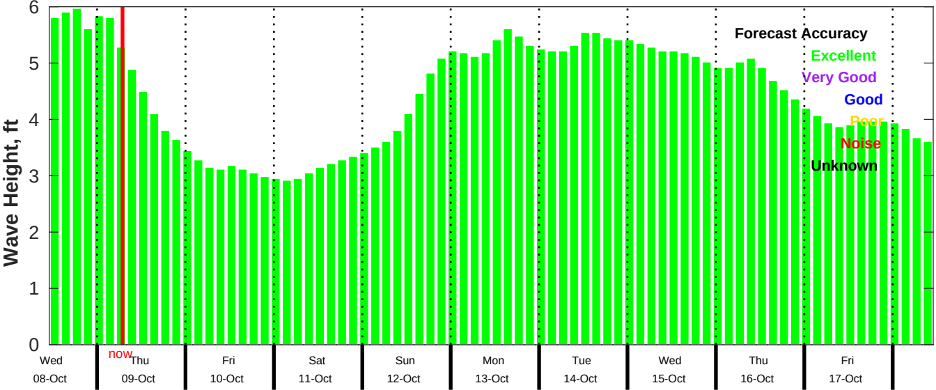
CMEMS Wave Forecast for NDBC 52211 from 07-Oct-2025 11:00:00 to 17-Oct-2025 11:00:00
