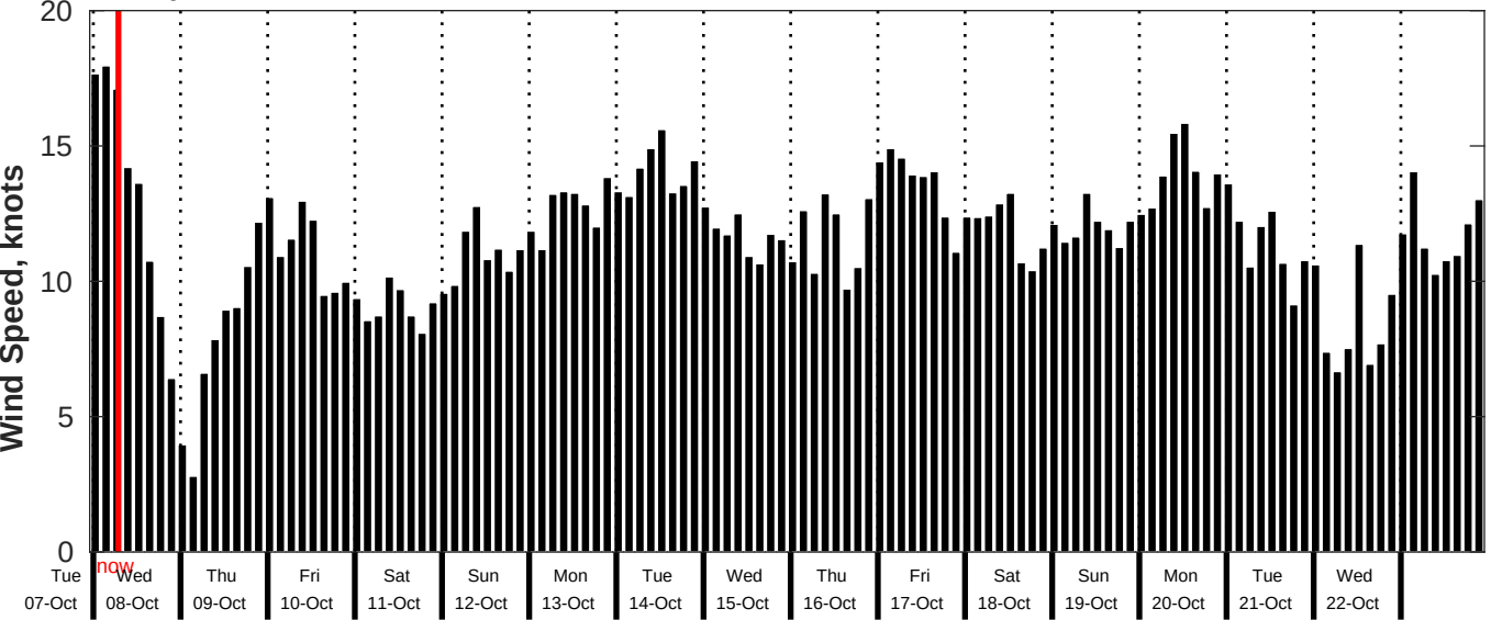
GFS Wind Speed Forecast for NDBC 52211 from 07-Oct-2025 23:00:00 to 23-Oct-2025 23:00:00
