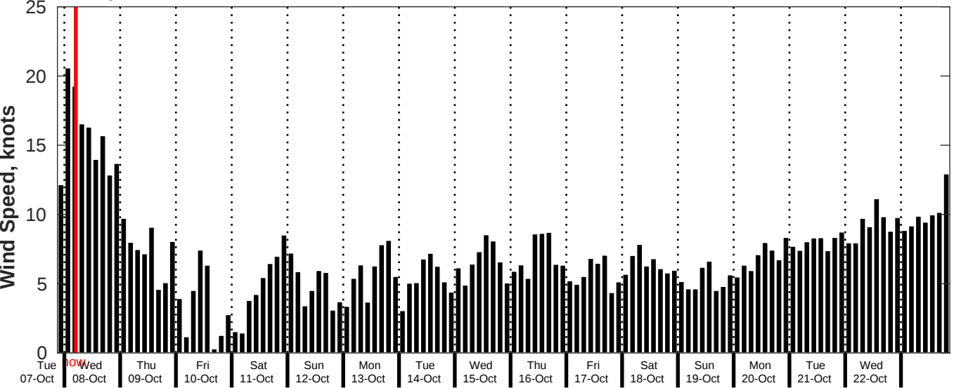
GFS Wind Speed Forecast for NDBC 52212 from 07-Oct-2025 21:00:00 to 23-Oct-2025 21:00:00
