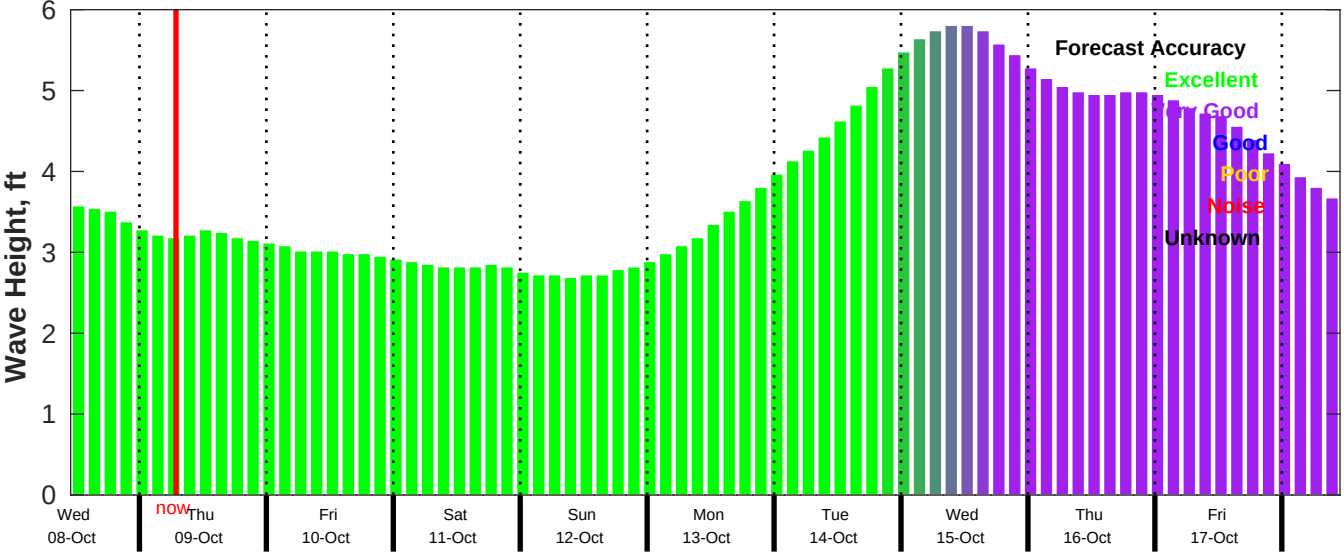
CMEMS Wave Forecast for NDBC 52213 from 07-Oct-2025 11:00:00 to 17-Oct-2025 11:00:00
