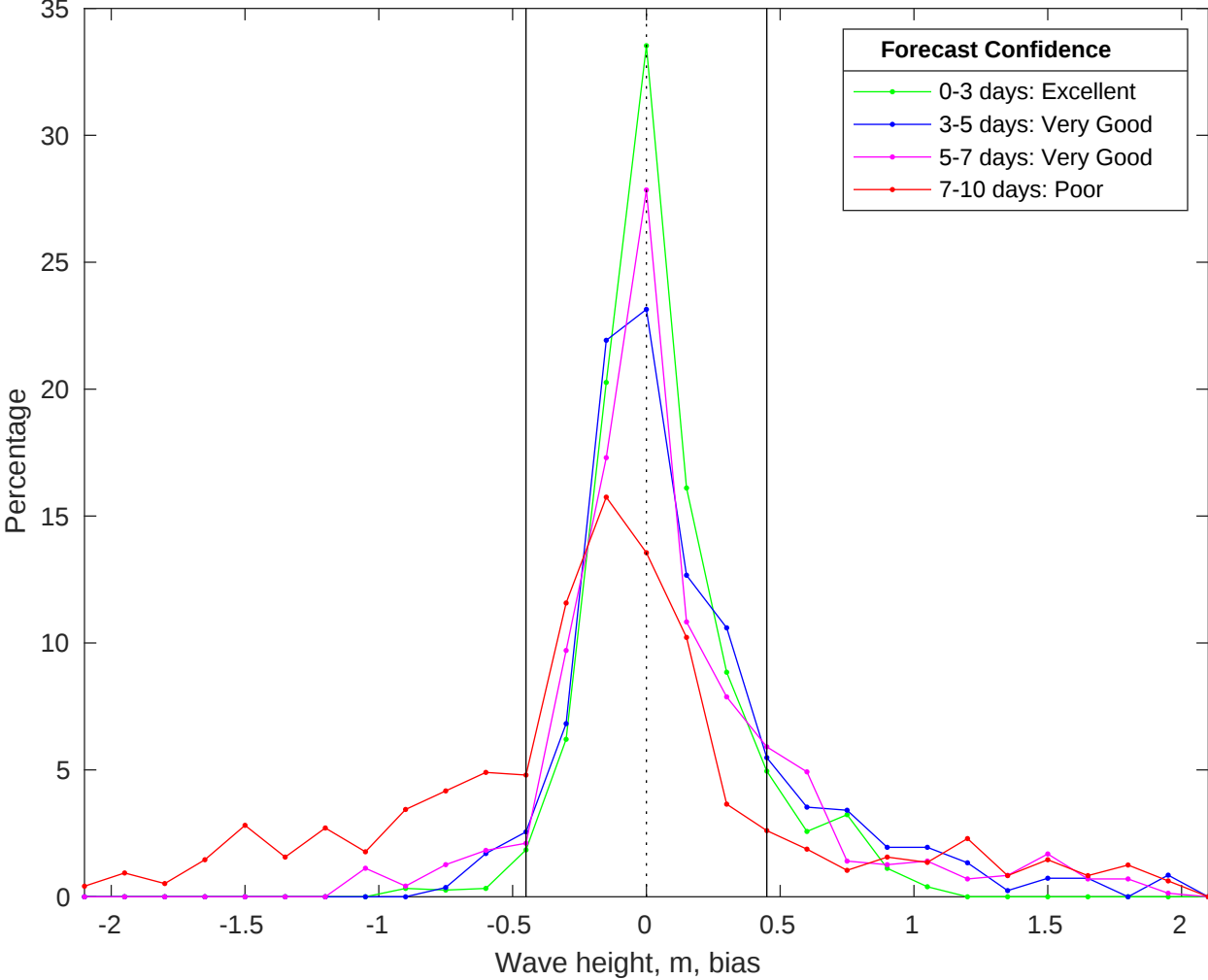
NDBC 41004 vs CMEMS Waves Bias Histogram: 09-Oct-2025
