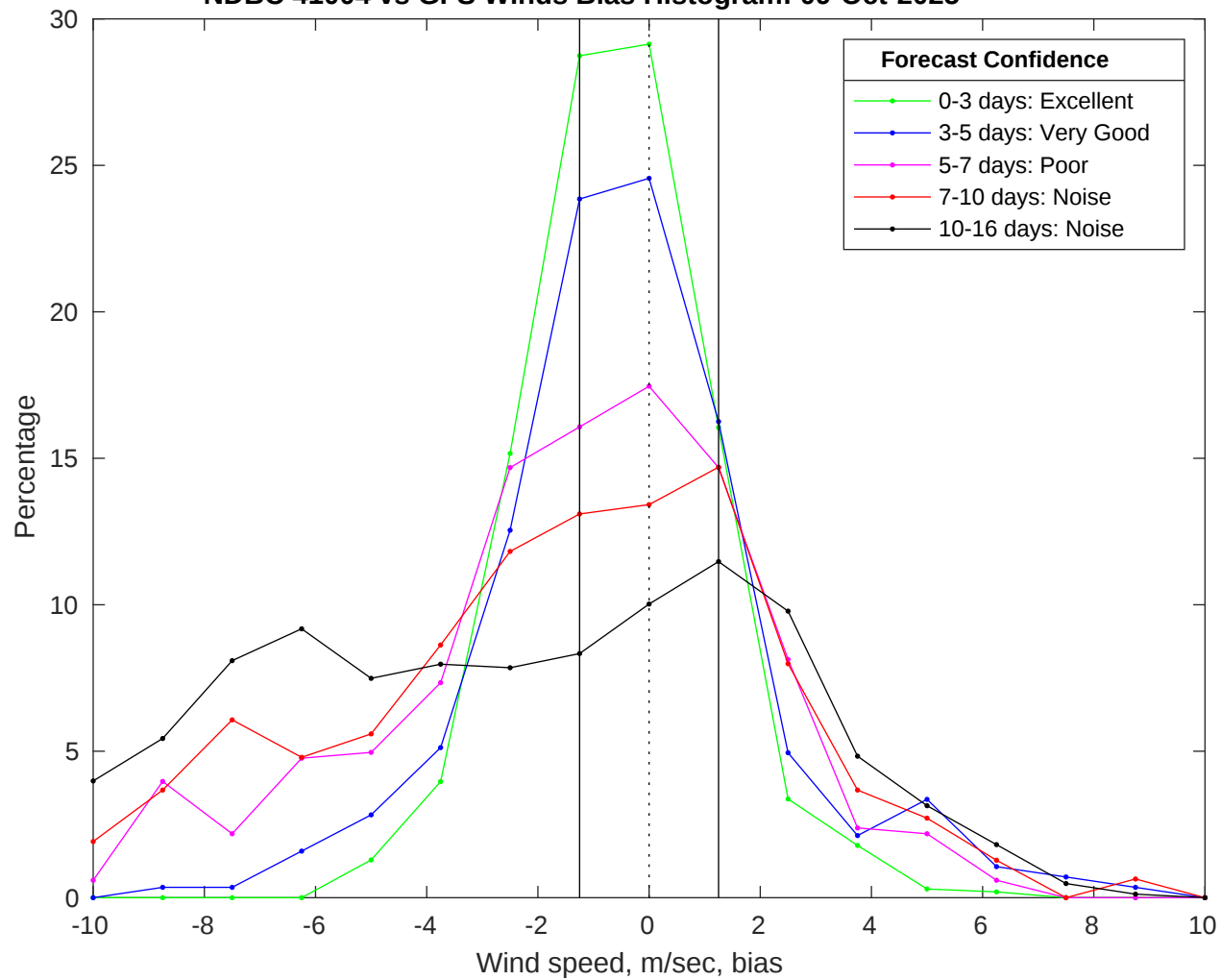
NDBC 41004 vs GFS Winds Bias Histogram: 09-Oct-2025
