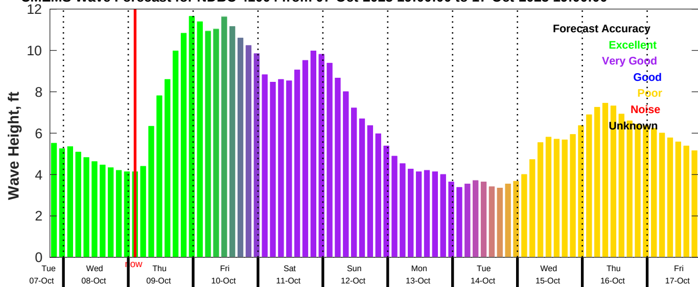
CMEMS Wave Forecast for NDBC 41004 from 07-Oct-2025 19:00:00 to 17-Oct-2025 19:00:00
