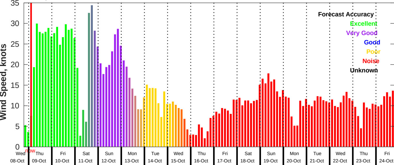
GFS Wind Speed Forecast for NDBC 41004 from 08-Oct-2025 19:00:00 to 24-Oct-2025 19:00:00
