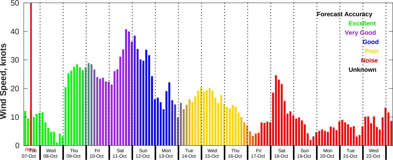
GFS Wind Speed Forecast for NDBC 41013 from 07-Oct-2025 07:00:00 to 23-Oct-2025 07:00:00
