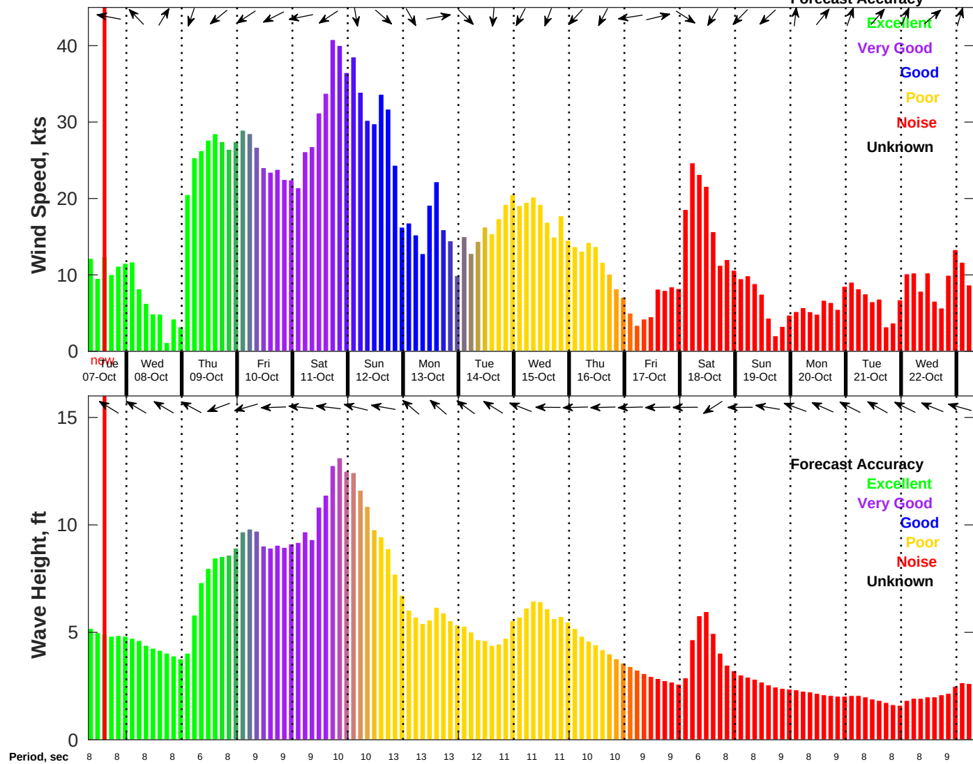
Wind & Wave Forecast for NDBC 41013 from 07-Oct-2025 07:00:00 to 23-Oct-2025 07:00:00
