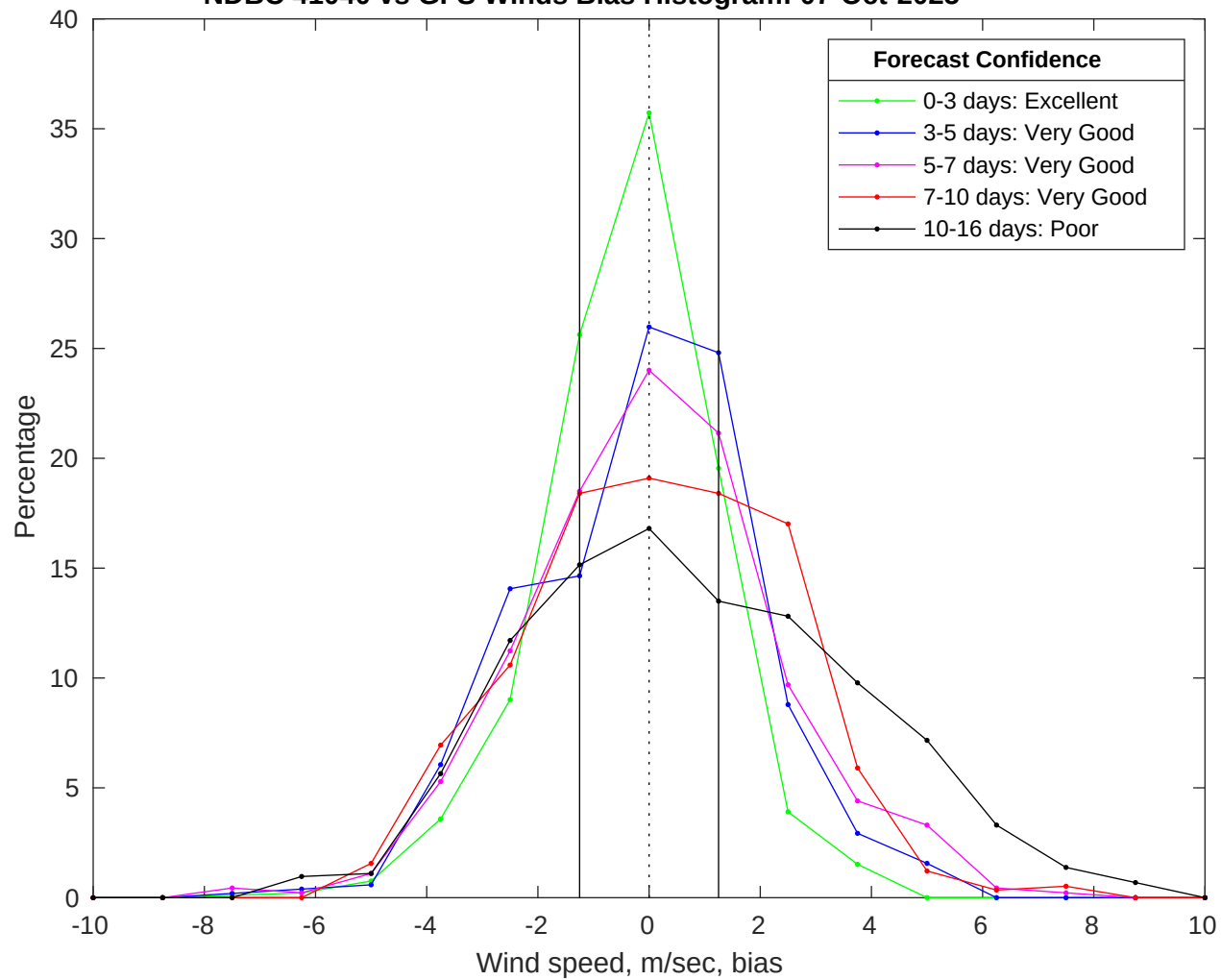
NDBC 41040 vs GFS Winds Bias Histogram: 07-Oct-2025
