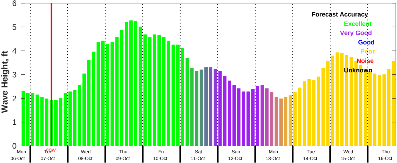
CMEMS Wave Forecast for NDBC 42019 from 06-Oct-2025 18:00:00 to 16-Oct-2025 18:00:00
