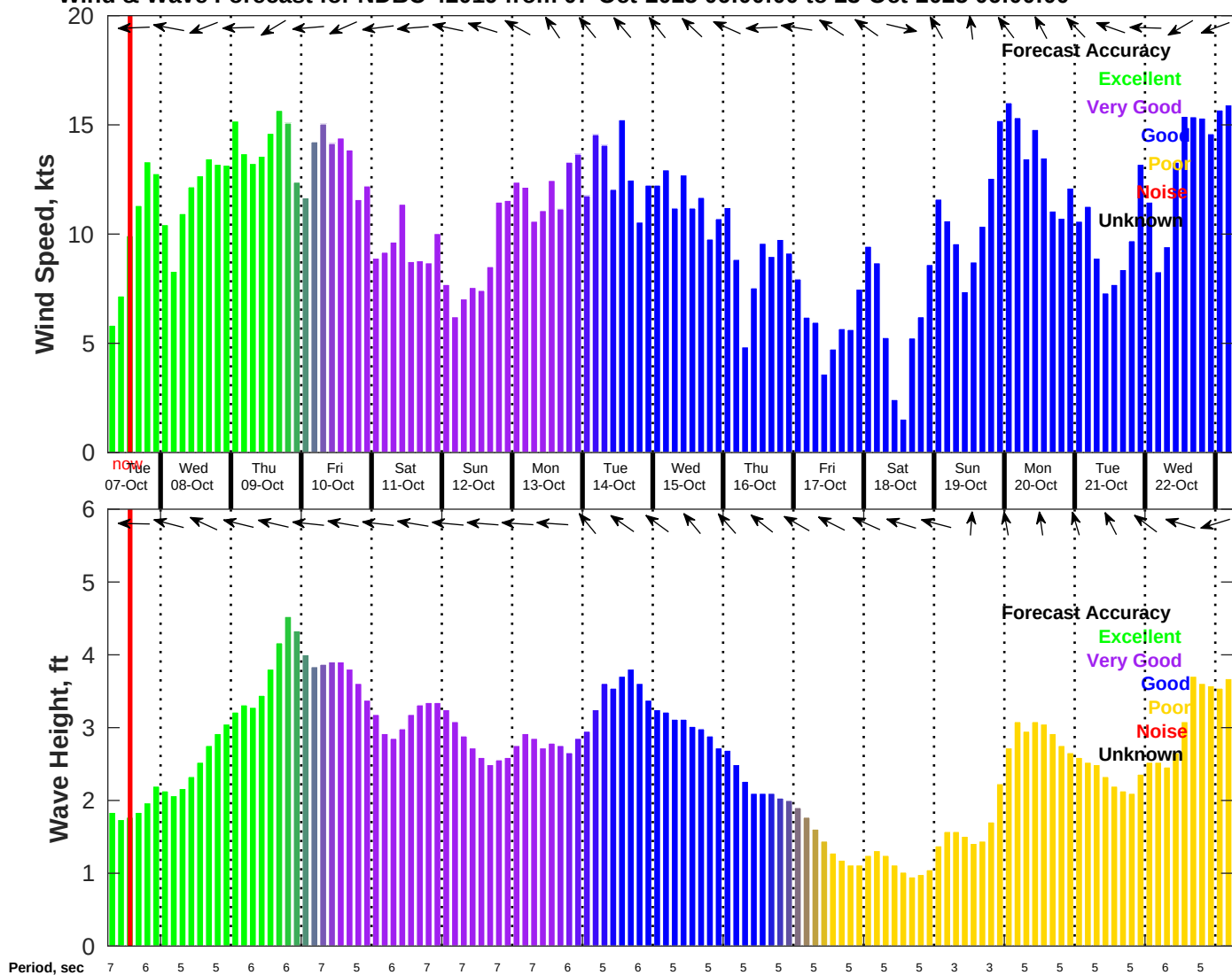
Wind & Wave Forecast for NDBC 42019 from 07-Oct-2025 06:00:00 to 23-Oct-2025 06:00:00
