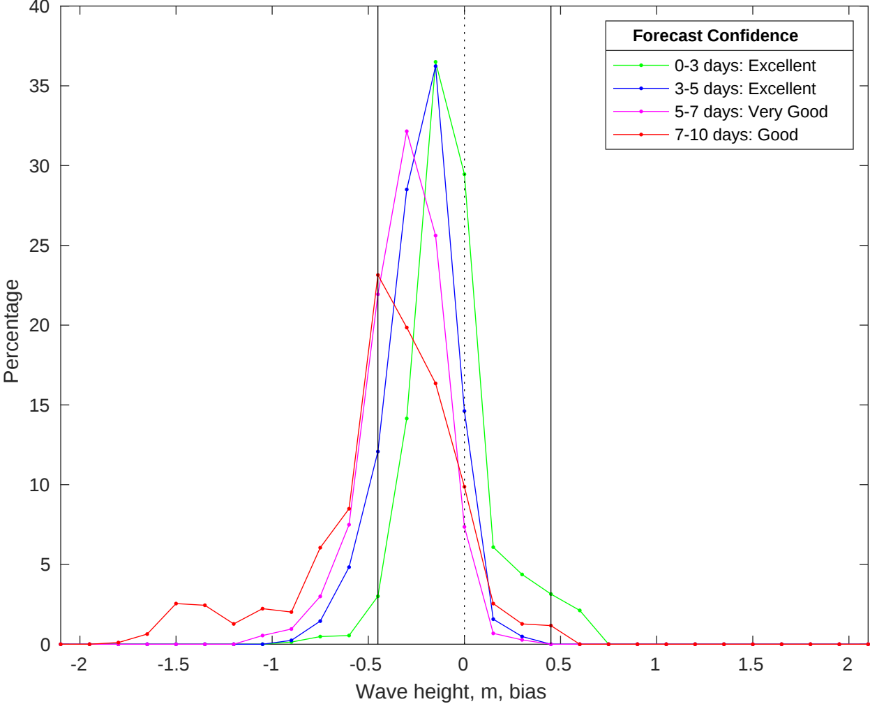
NDBC 42020 vs CMEMS Waves Bias Histogram: 07-Oct-2025
