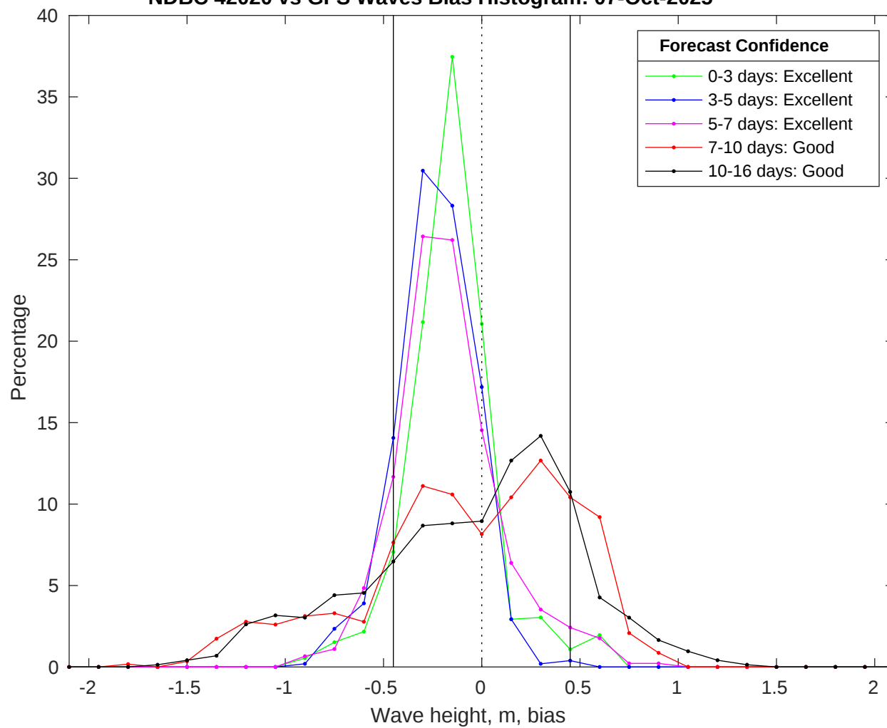
NDBC 42020 vs GFS Waves Bias Histogram: 07-Oct-2025
