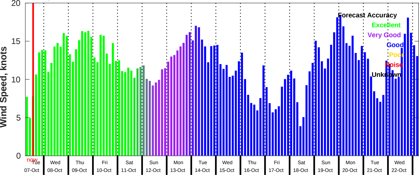
GFS Wind Speed Forecast for NDBC 42020 from 07-Oct-2025 06:00:00 to 23-Oct-2025 06:00:00
