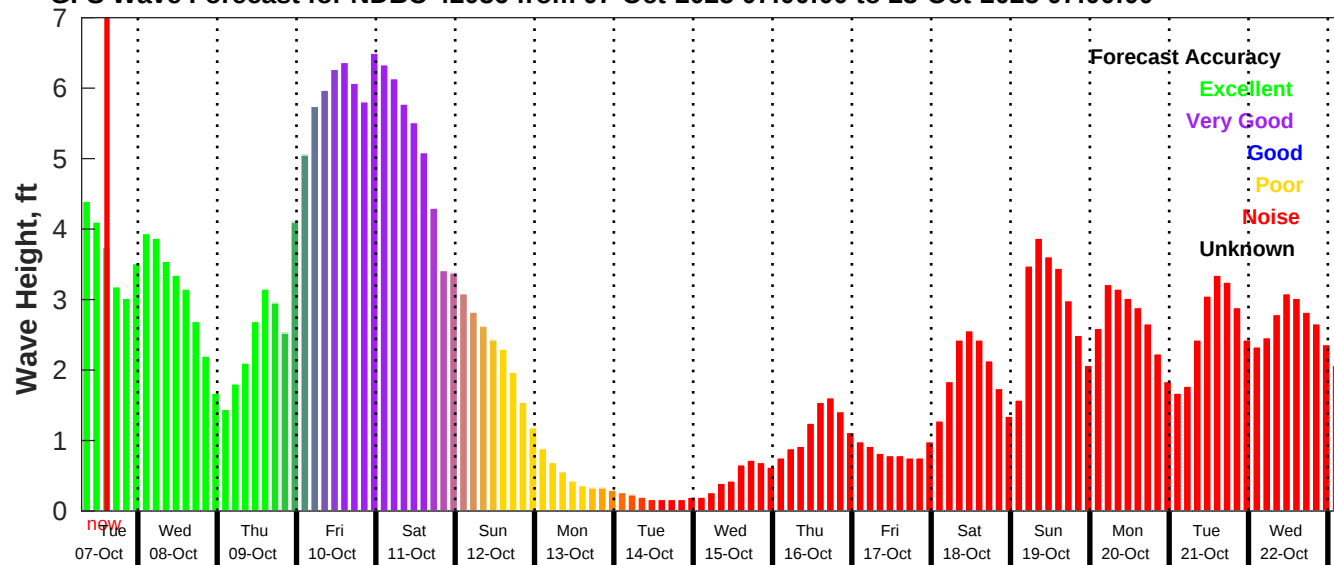
GFS Wave Forecast for NDBC 42036 from 07-Oct-2025 07:00:00 to 23-Oct-2025 07:00:00
