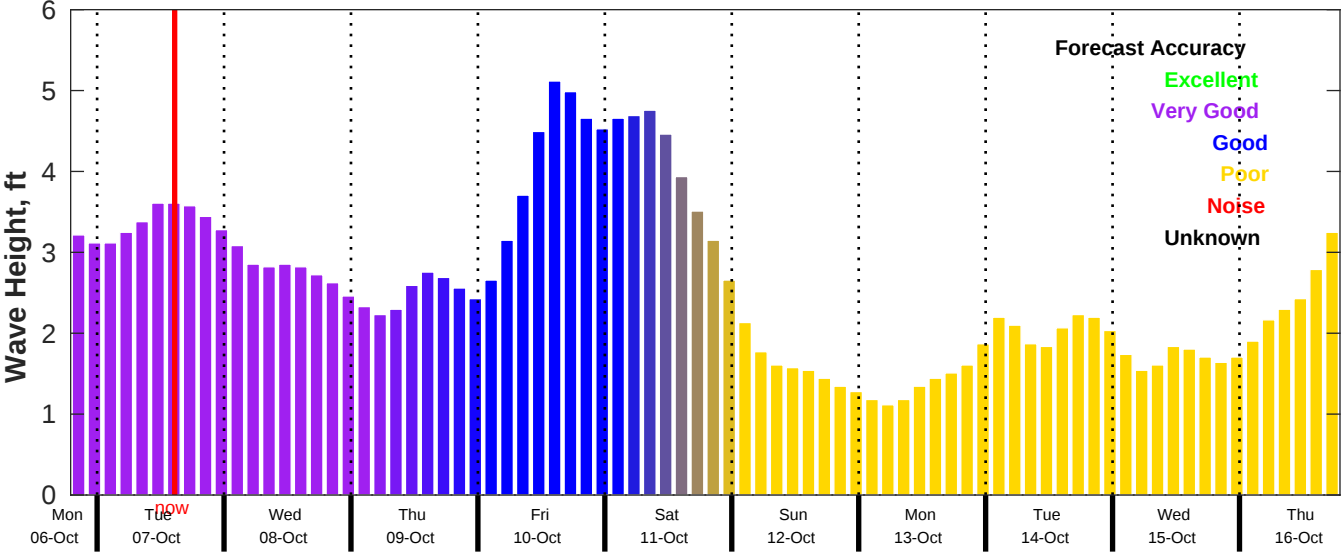
CMEMS Wave Forecast for NDBC 42040 from 06-Oct-2025 19:00:00 to 16-Oct-2025 19:00:00
