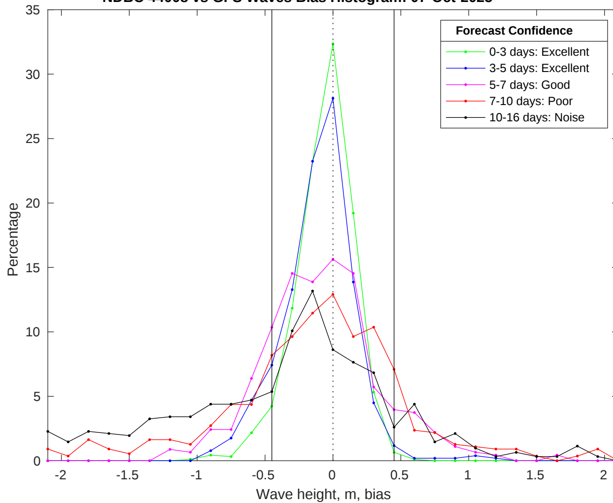
NDBC 44008 vs GFS Waves Bias Histogram: 07-Oct-2025
