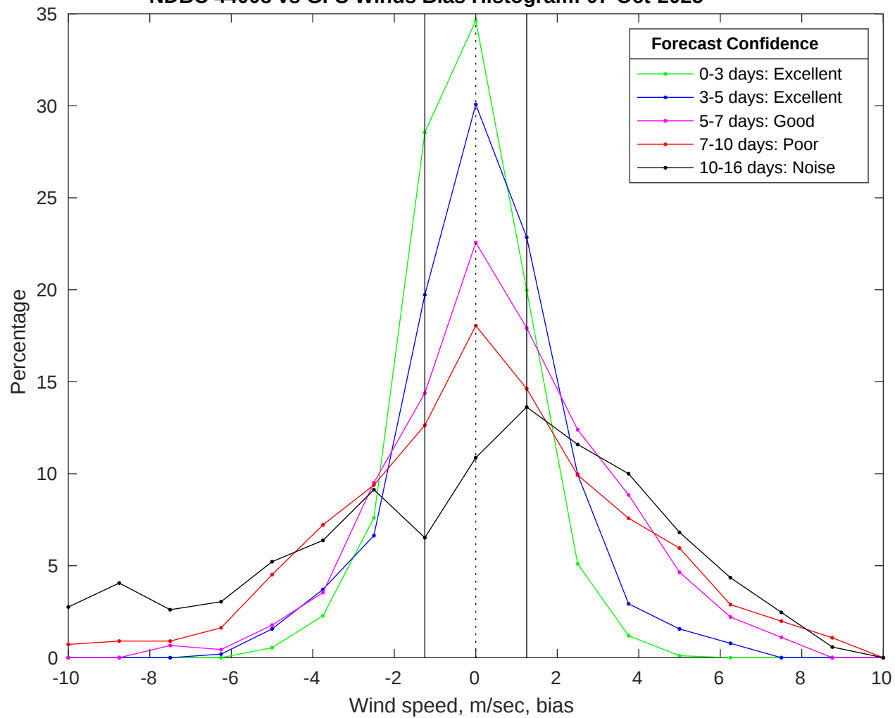
NDBC 44008 vs GFS Winds Bias Histogram: 07-Oct-2025
