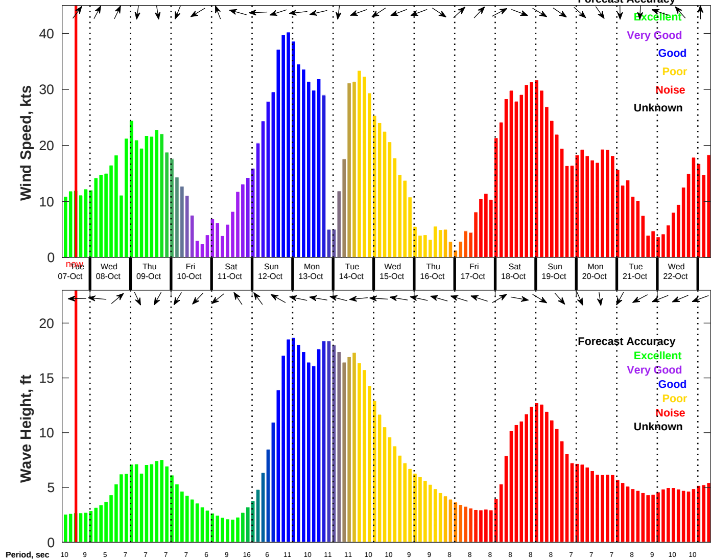
Wind & Wave Forecast for NDBC 44008 from 07-Oct-2025 08:00:00 to 23-Oct-2025 08:00:00
