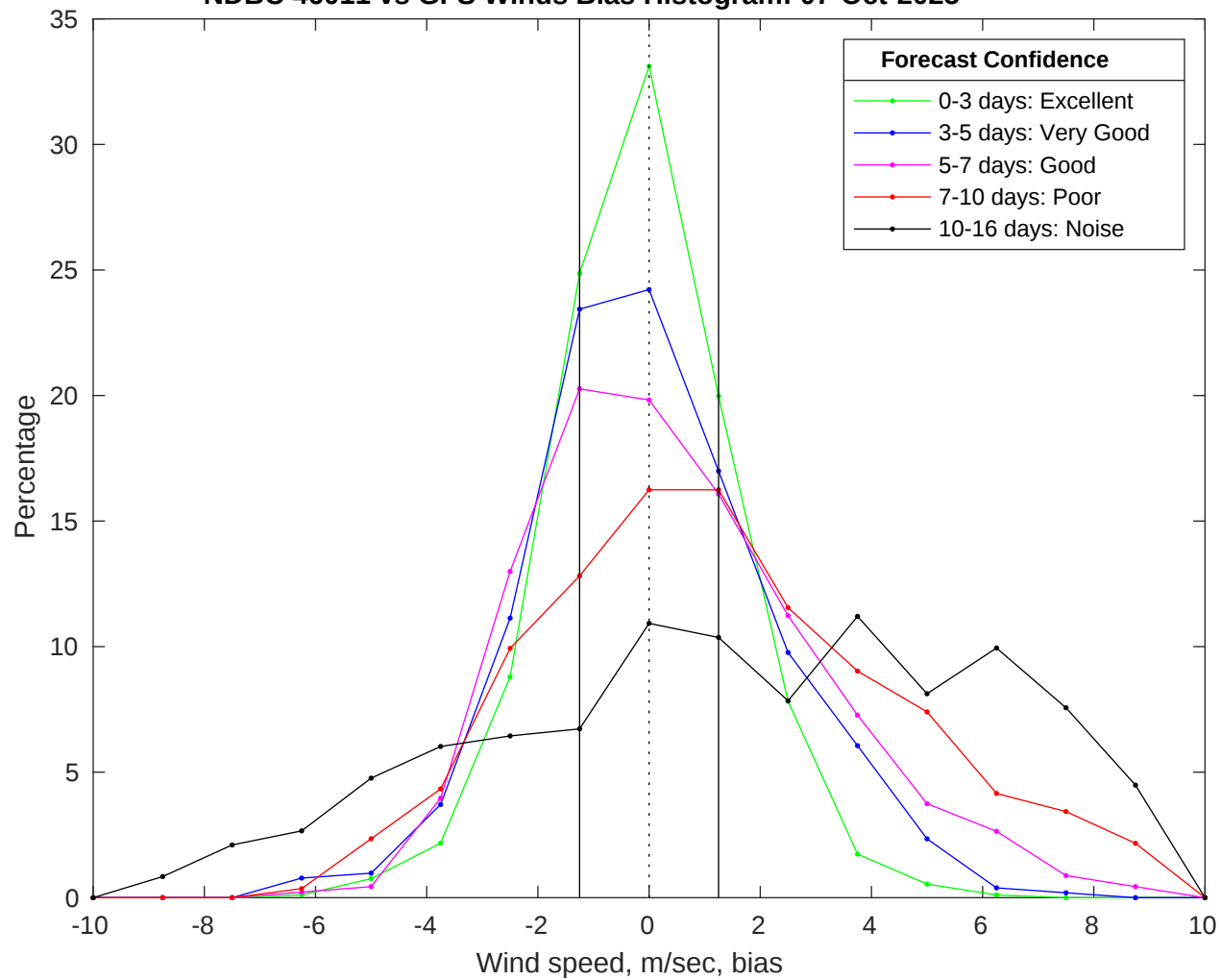
NDBC 46011 vs GFS Winds Bias Histogram: 07-Oct-2025
