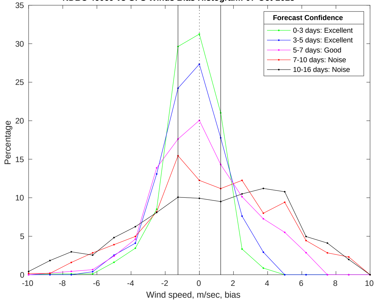
NDBC 46069 vs GFS Winds Bias Histogram: 07-Oct-2025
