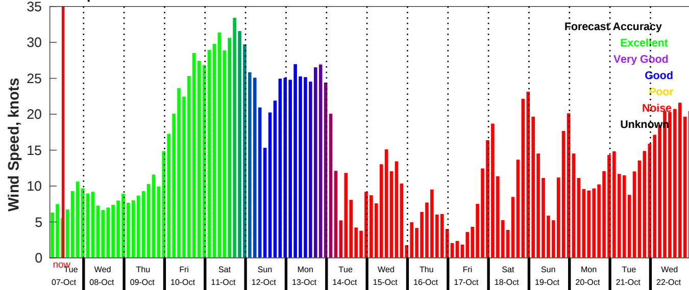
GFS Wind Speed Forecast for NDBC 46069 from 07-Oct-2025 04:00:00 to 23-Oct-2025 04:00:00
