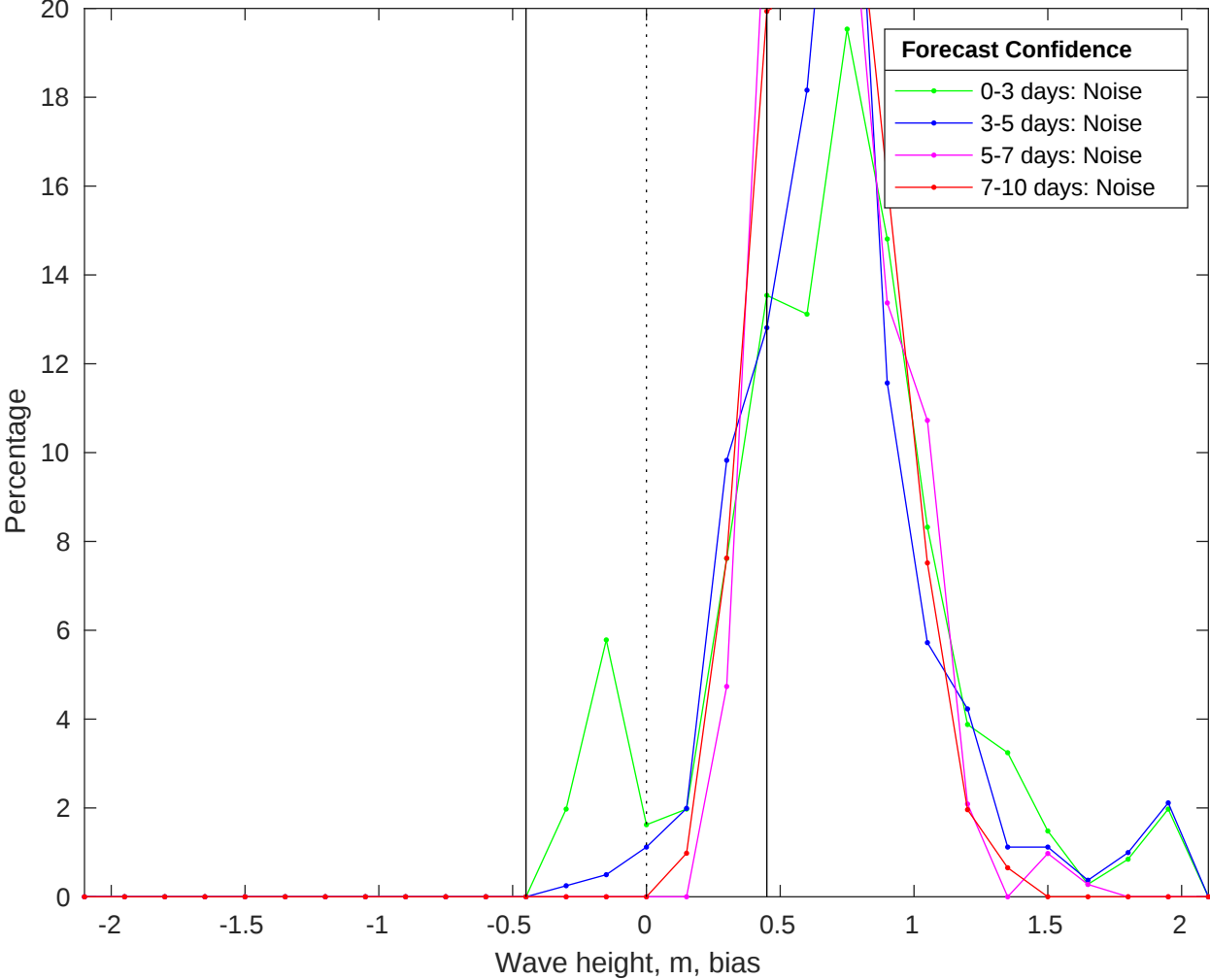
NDBC 51211 vs CMEMS Waves Bias Histogram: 07-Oct-2025
