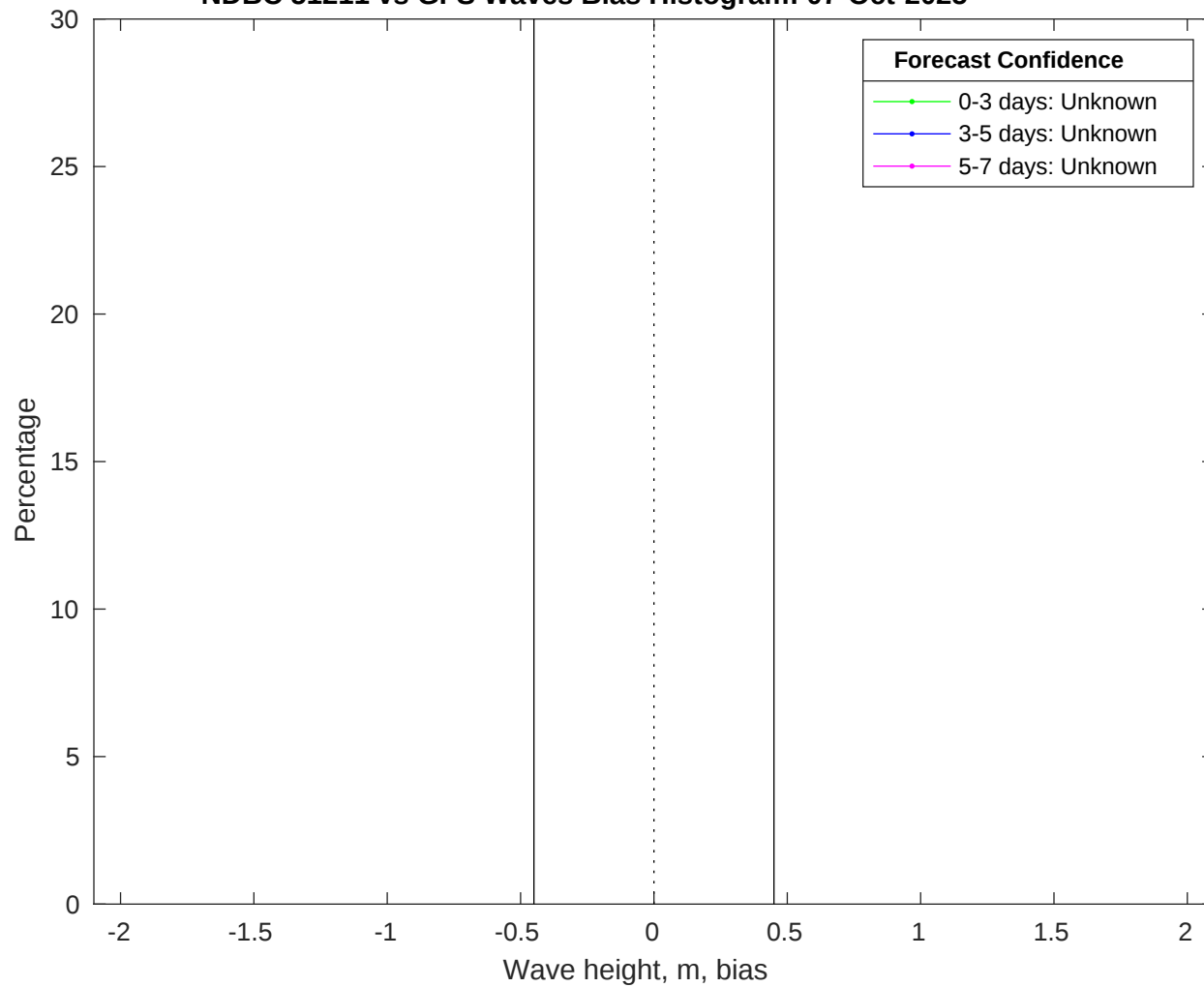
NDBC 51211 vs GFS Waves Bias Histogram: 07-Oct-2025
