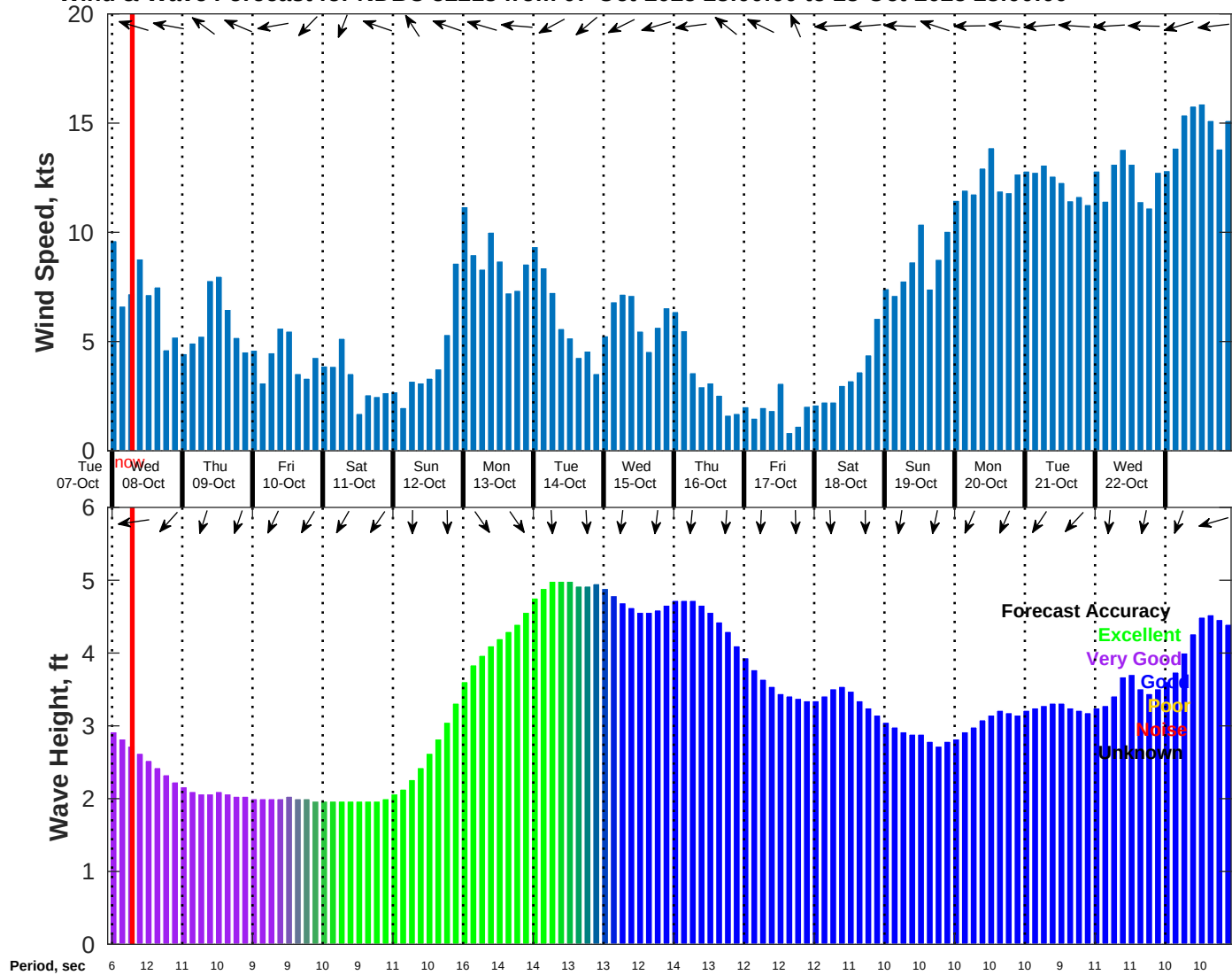
Wind & Wave Forecast for NDBC 52213 from 07-Oct-2025 23:00:00 to 23-Oct-2025 23:00:00
