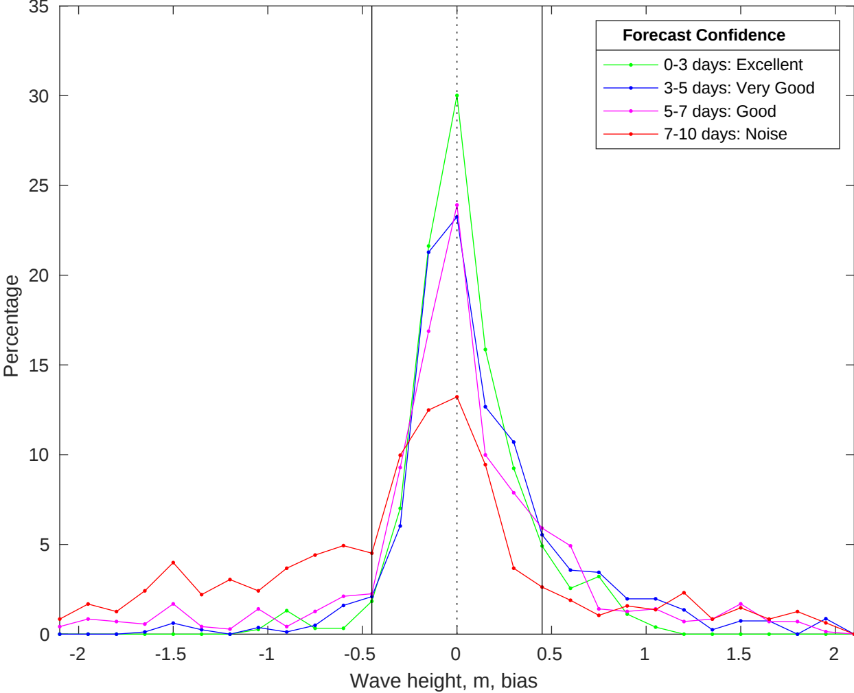
NDBC 41004 vs CMEMS Waves Bias Histogram: 10-Oct-2025
