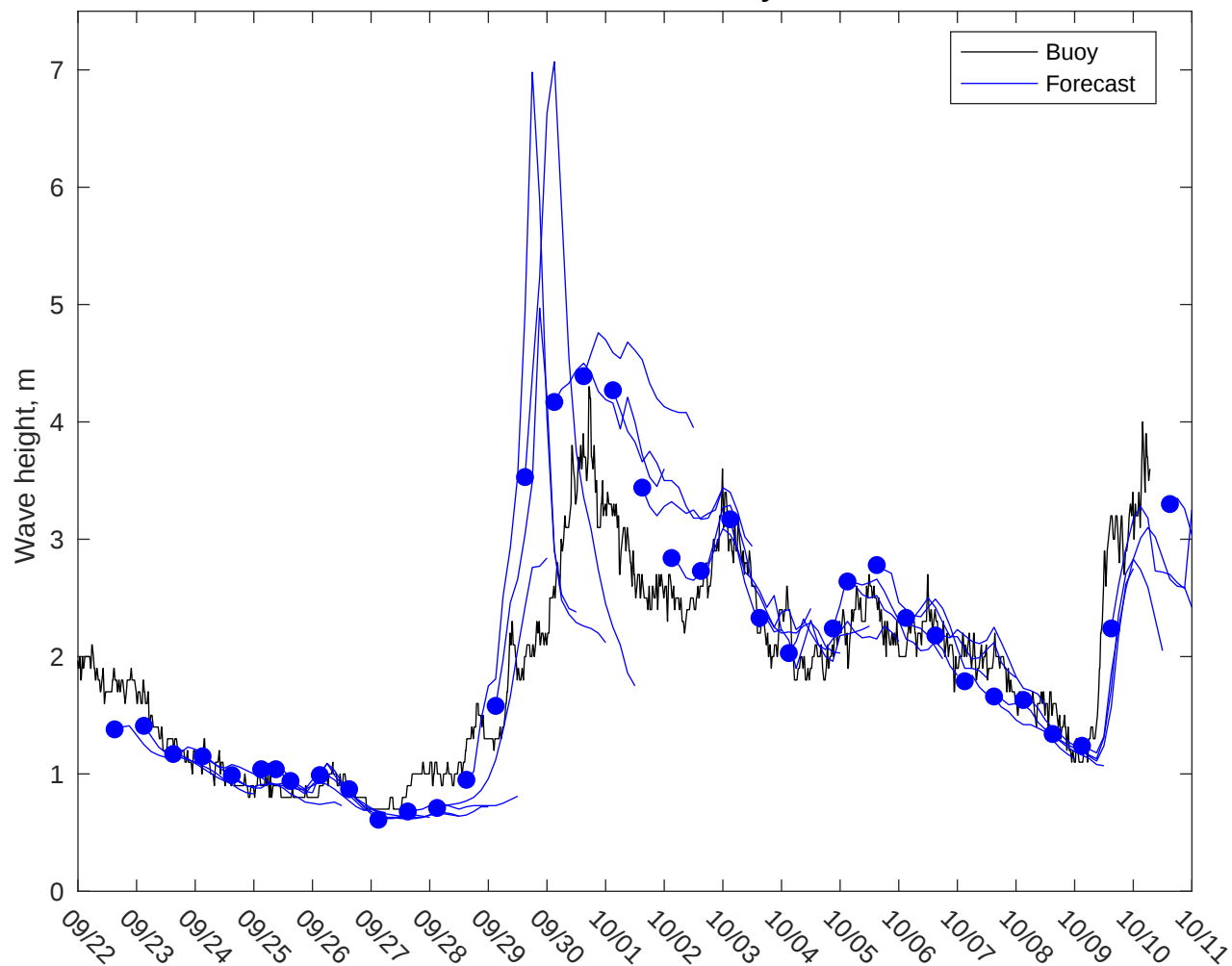
NDBC 41004 vs GFS Waves: 3 to 5 day forecast
