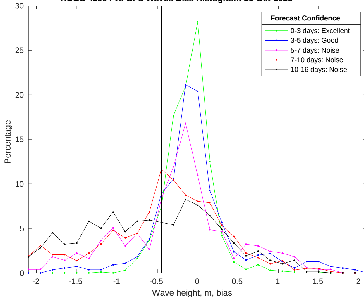
NDBC 41004 vs GFS Waves Bias Histogram: 10-Oct-2025
