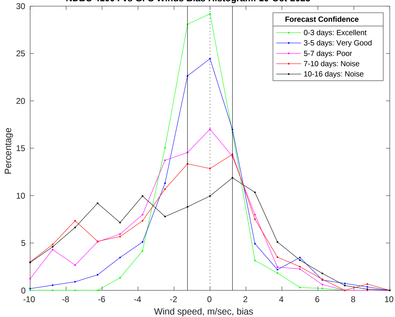
NDBC 41004 vs GFS Winds Bias Histogram: 10-Oct-2025
