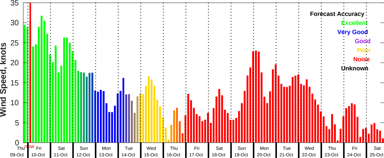
GFS Wind Speed Forecast for NDBC 41004 from 09-Oct-2025 19:00:00 to 25-Oct-2025 19:00:00
