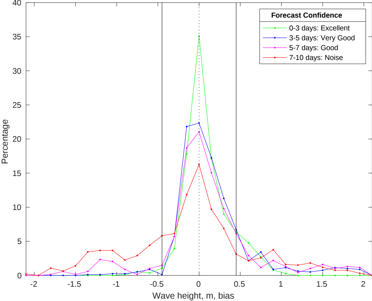
NDBC 41013 vs CMEMS Waves Bias Histogram: 10-Oct-2025
