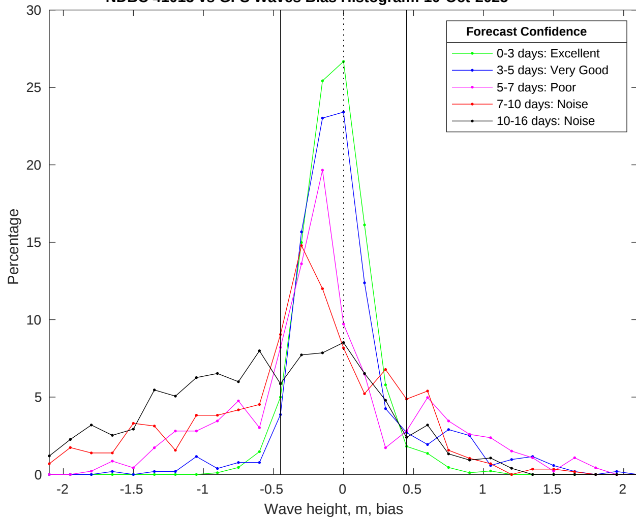
NDBC 41013 vs GFS Waves Bias Histogram: 10-Oct-2025
