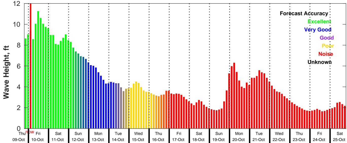
GFS Wave Forecast for NDBC 41013 from 09-Oct-2025 19:00:00 to 25-Oct-2025 19:00:00
