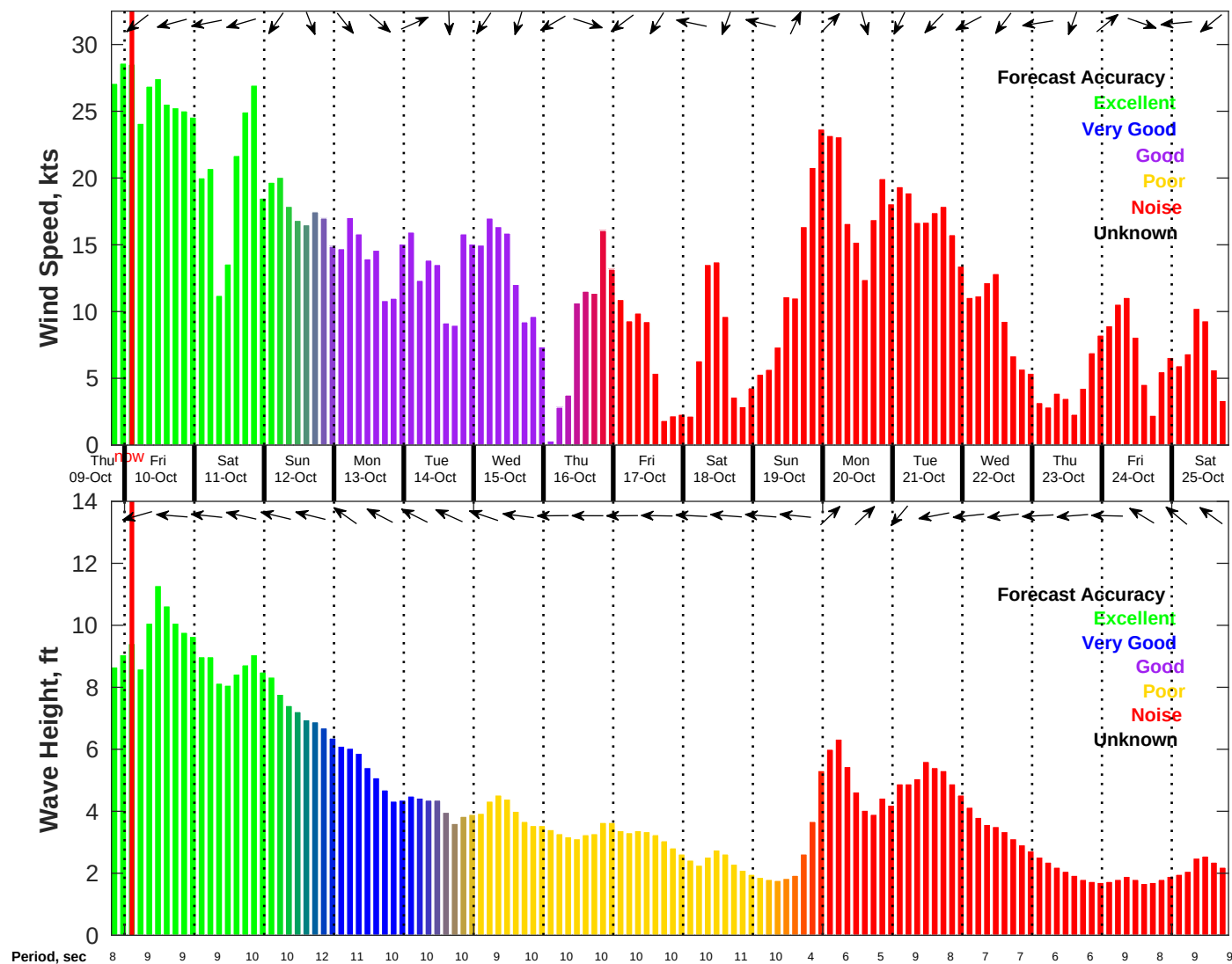
Wind & Wave Forecast for NDBC 41013 from 09-Oct-2025 19:00:00 to 25-Oct-2025 19:00:00
