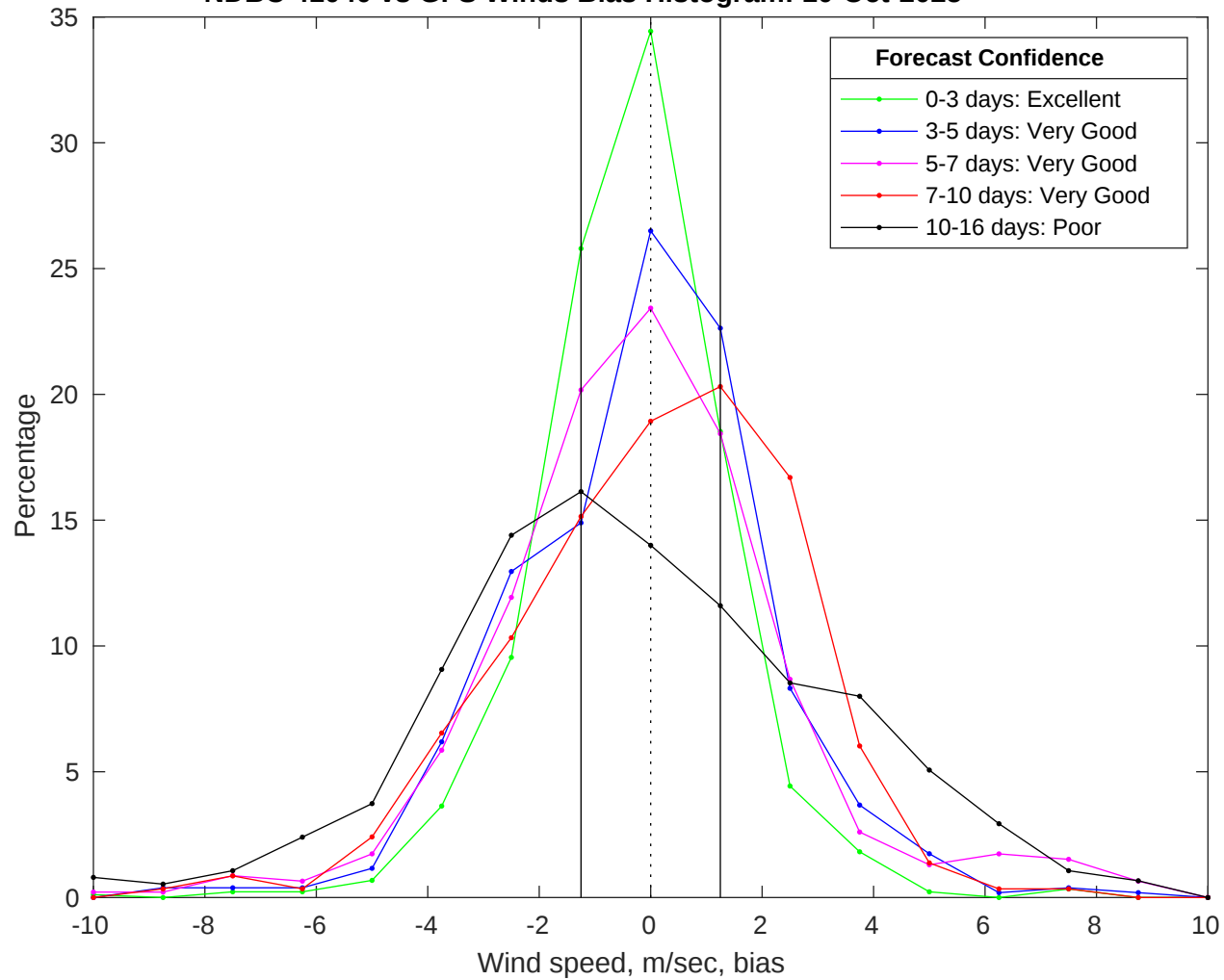
NDBC 41040 vs GFS Winds Bias Histogram: 10-Oct-2025
