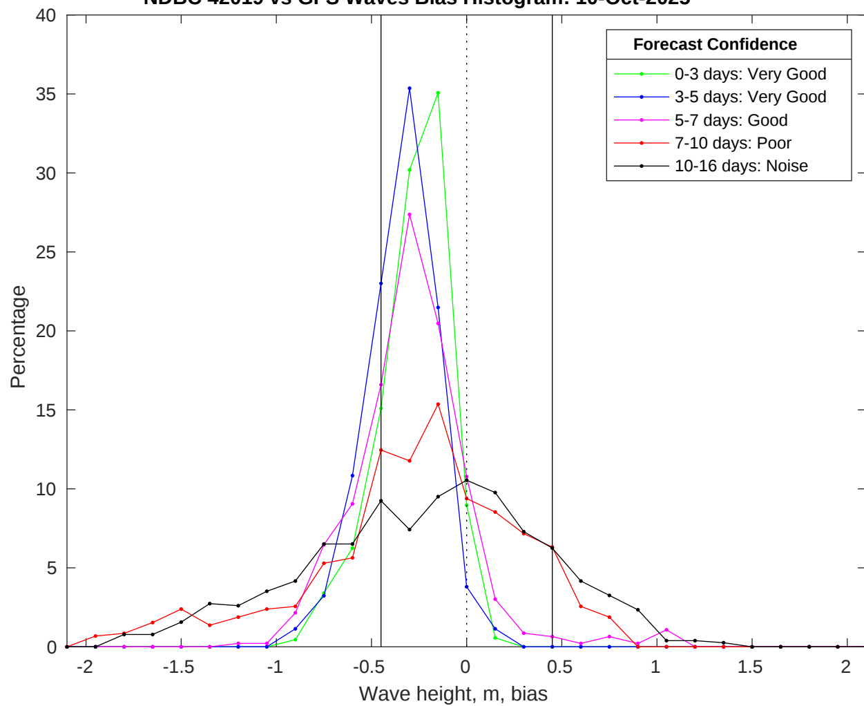
NDBC 42019 vs GFS Waves Bias Histogram: 10-Oct-2025
