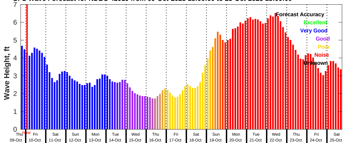
GFS Wave Forecast for NDBC 42019 from 09-Oct-2025 18:00:00 to 25-Oct-2025 18:00:00
