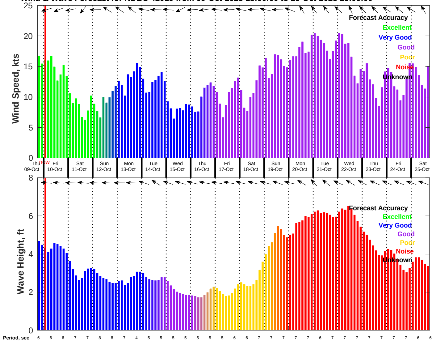
Wind & Wave Forecast for NDBC 42019 from 09-Oct-2025 18:00:00 to 25-Oct-2025 18:00:00
