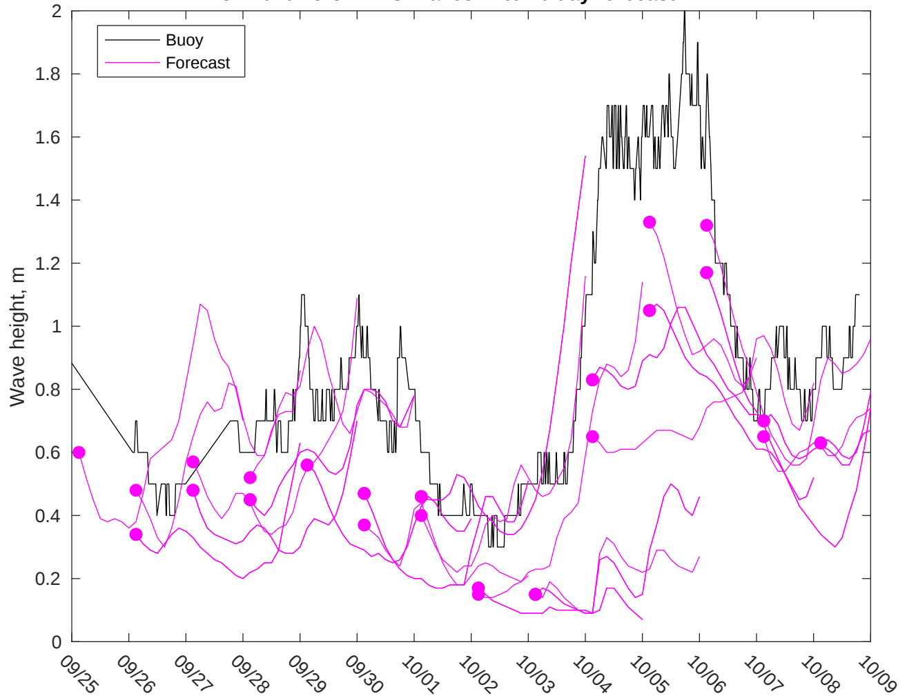
NDBC 42020 vs CMEMS Waves: 7 to 10 day forecast
