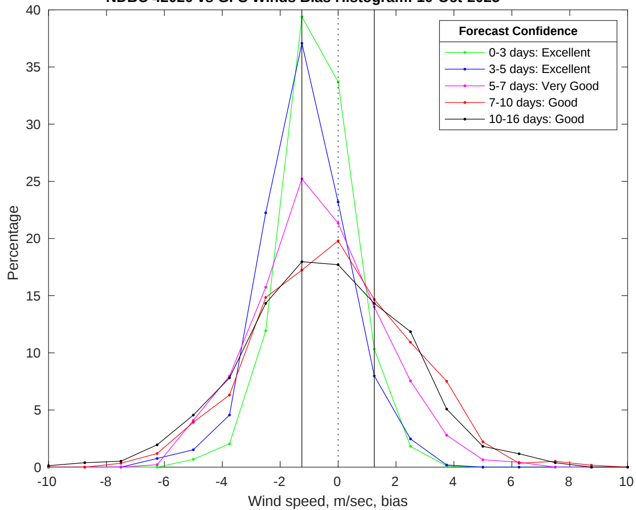
NDBC 42020 vs GFS Winds Bias Histogram: 10-Oct-2025
