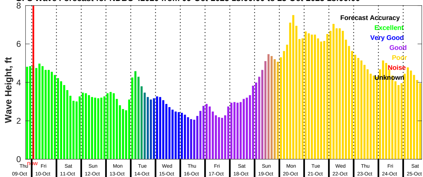
GFS Wave Forecast for NDBC 42020 from 09-Oct-2025 18:00:00 to 25-Oct-2025 18:00:00
