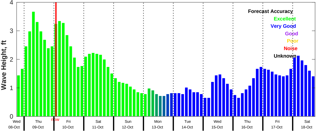
CMEMS Wave Forecast for NDBC 42035 from 08-Oct-2025 18:00:00 to 18-Oct-2025 18:00:00
