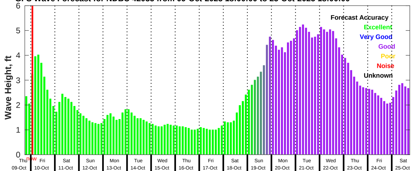
GFS Wave Forecast for NDBC 42035 from 09-Oct-2025 18:00:00 to 25-Oct-2025 18:00:00
