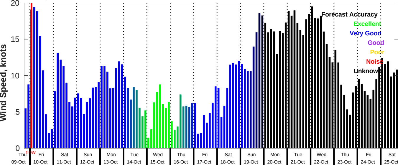
GFS Wind Speed Forecast for NDBC 42035 from 09-Oct-2025 18:00:00 to 25-Oct-2025 18:00:00
